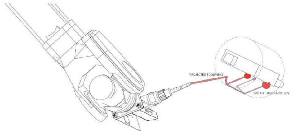
Fig. 8: Toolpaths are projected in real time, providing indication to the human operator where the robot will move next (path weight and colour) and how long it will melt in a given location (sphere radii).
