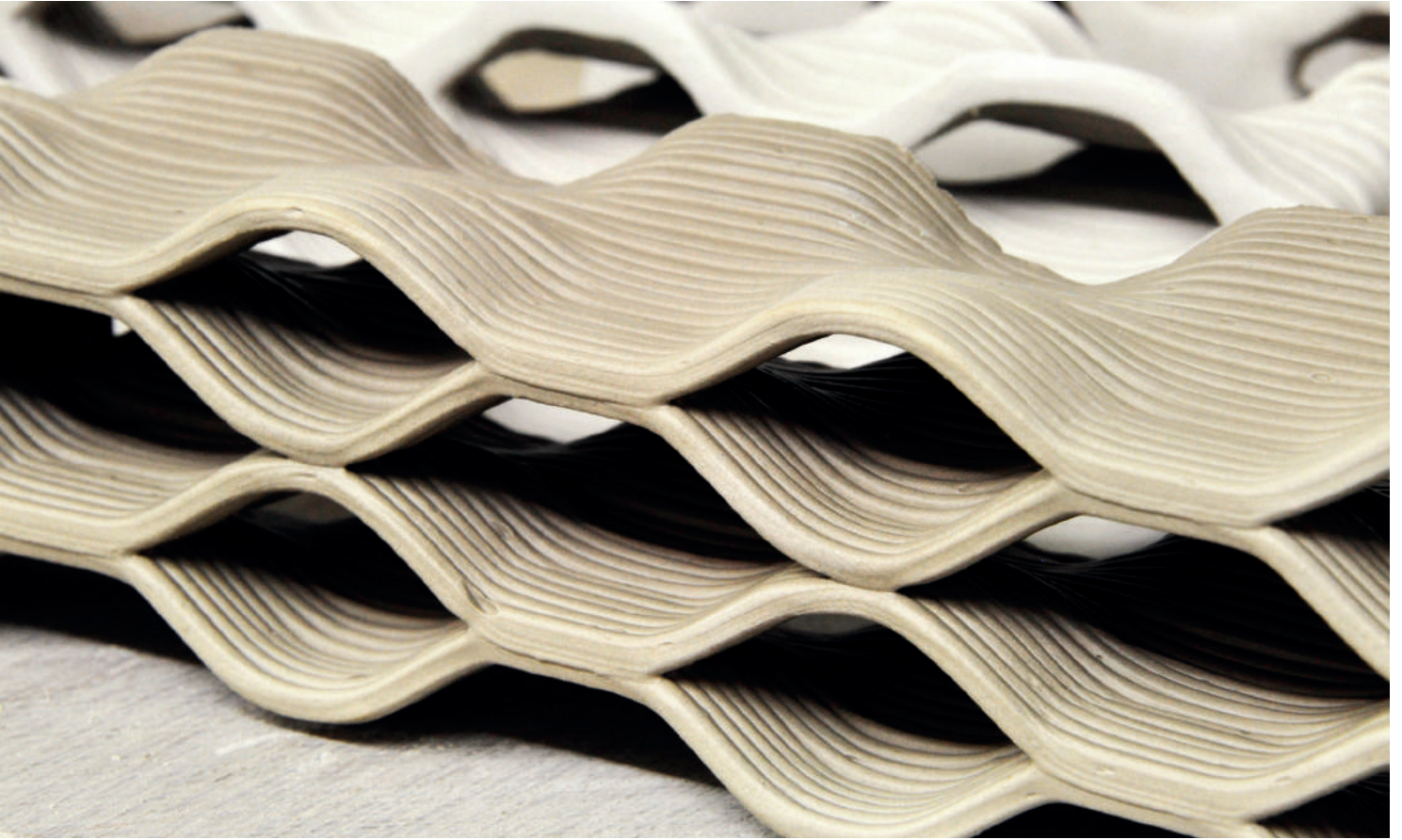
Fig. 14: Honeycomb brick: detail.
