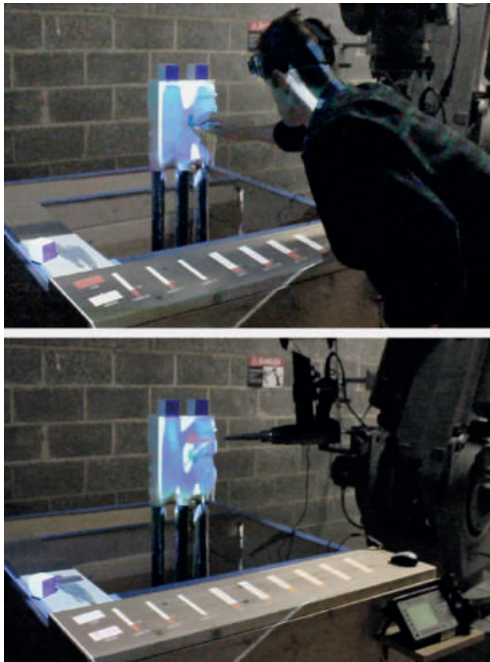
Fig. 7: Above: Desired void areas are physically indicated using a coloured marker. Below: The virtual model is automatically reconfigured around the indicated opening and the robot proceeds to melt away this area.
